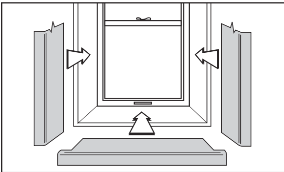
Option 1. Notching the sill panel only.
