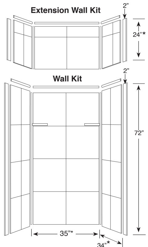
Shown with F3636 Shower Base, X3662 Extension Wall Kit
