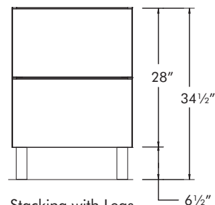
Stacking with Legs Required Hardware: VFSTACKA or VFSTACKL
