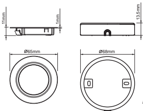
Recessed: Cut out size: Ø60mm
