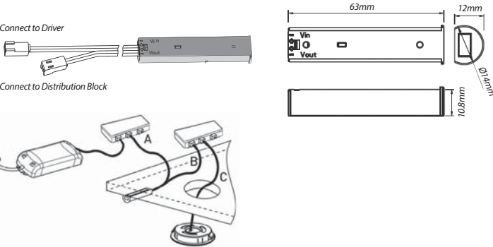
Image shows how this product is set up
