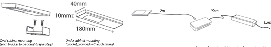
Cables, Connectors and Accessories
