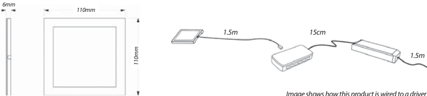
Image shows how this product is wired to a driver
