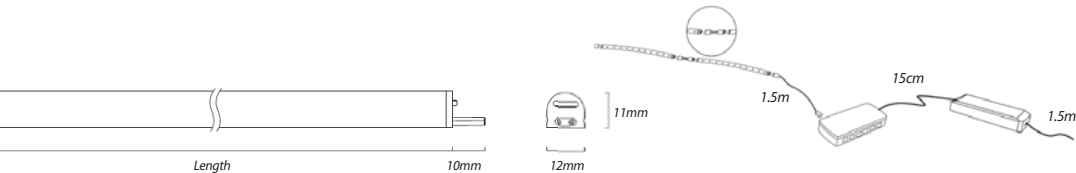
Image shows how this product is wired to a driver
