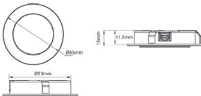
Recessed: Cut out size: Ø59-61mm
