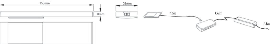
Image shows how this product is wired to a driver
