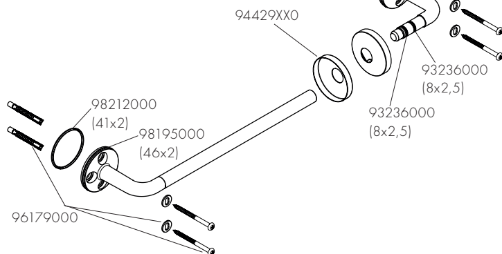
AXOR Universal Circular 42813XX0
