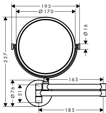
AXOR Universal Circular 42849XXX
