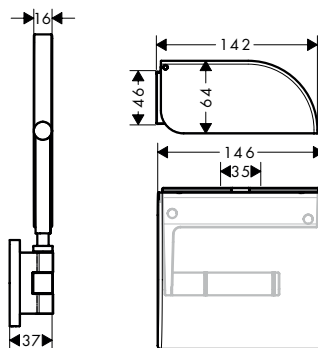
AXOR Universal Circular 42858XXX
