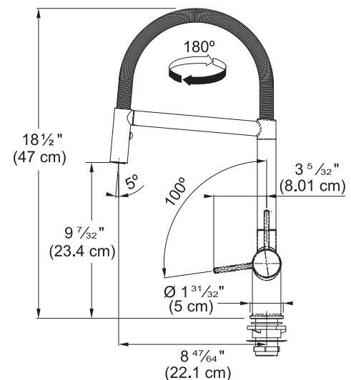
Dimensional Drawing
